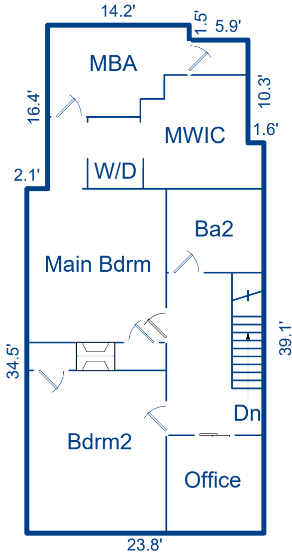
Second Floor 1149.3 sf
